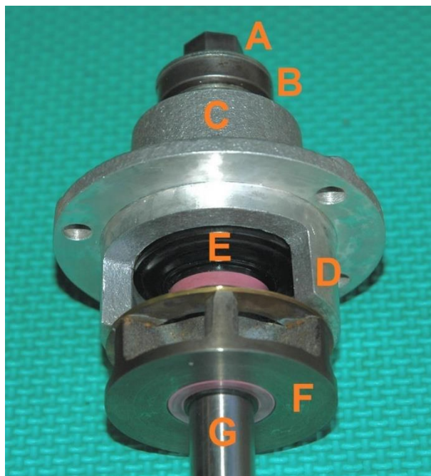
Above: Figure 12. A repeat of Figure 1, showing Item Numbers that are referred to in the text.
