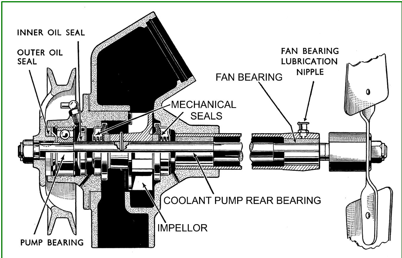
Above: Cross section of a coolant pump with some changes incorporated.
