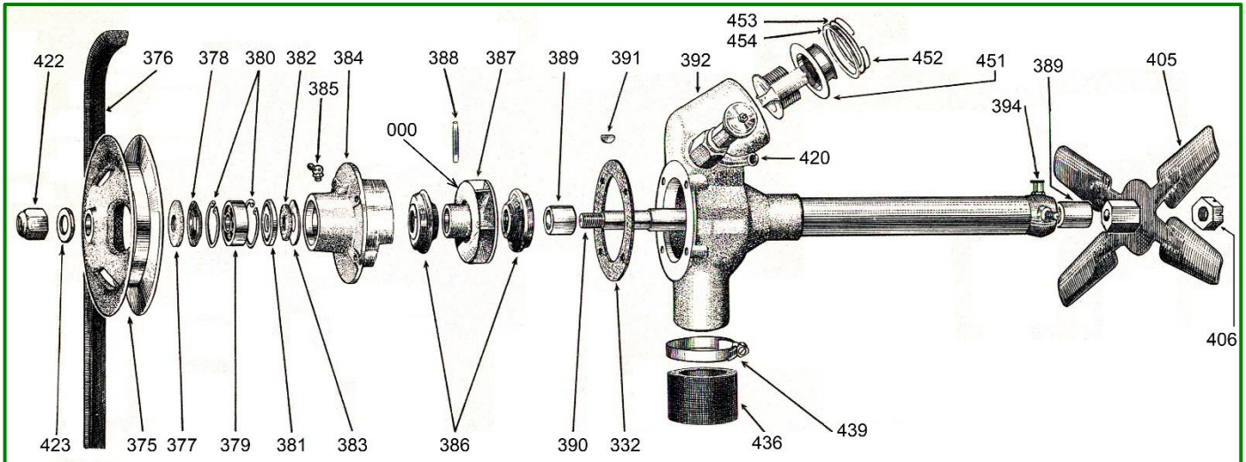
Above: Figure 1. Illustration taken from the Spare Parts Catalogue, dated May, 1952.
