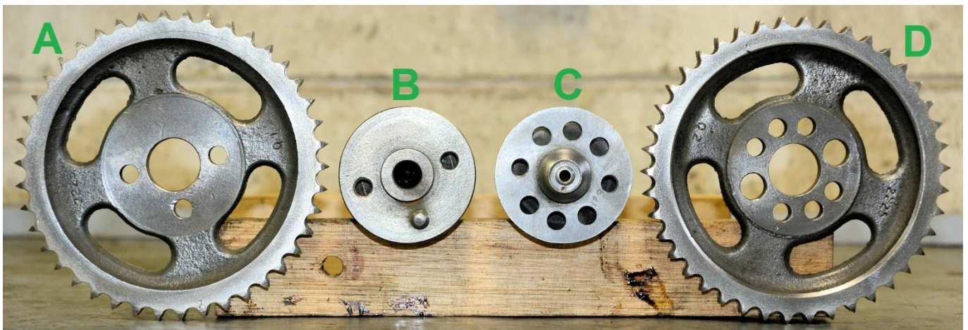
Above: Figure 26. Where – ‘A’ is early chainwheel, ‘B’ is early camshaft, ‘C’ is later camshaft, and ‘D’ is later chainwheel. Item ‘C’ has been running with incorrect end float adjustment.
