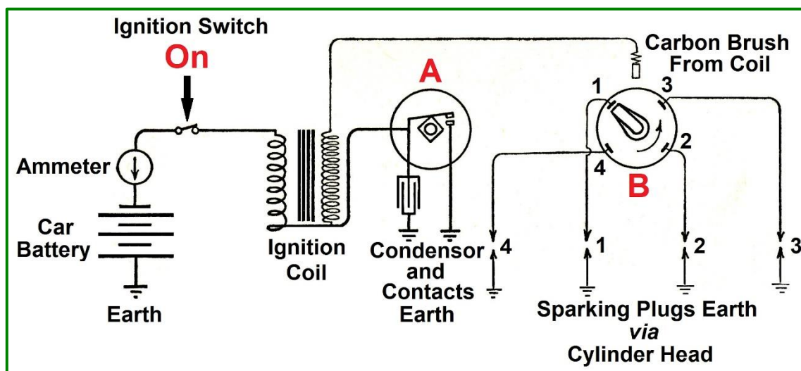
Above: Figure 52. Basic diagram of ignition circuit as used with the Jowett engine.
